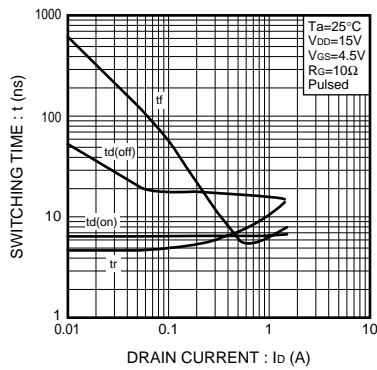
Fig.1 Switching Characteristics
