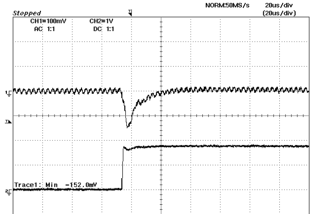
Figure 22: Typical transient response to step load change at 2.5A/\mu S from 50% to 100% of I_o , max at 5V_{in} , 1.8V_{out} ( C_{out} = 1\mu F ceramic, 10\mu F tantalum)
