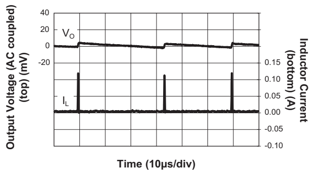
Output Ripple
