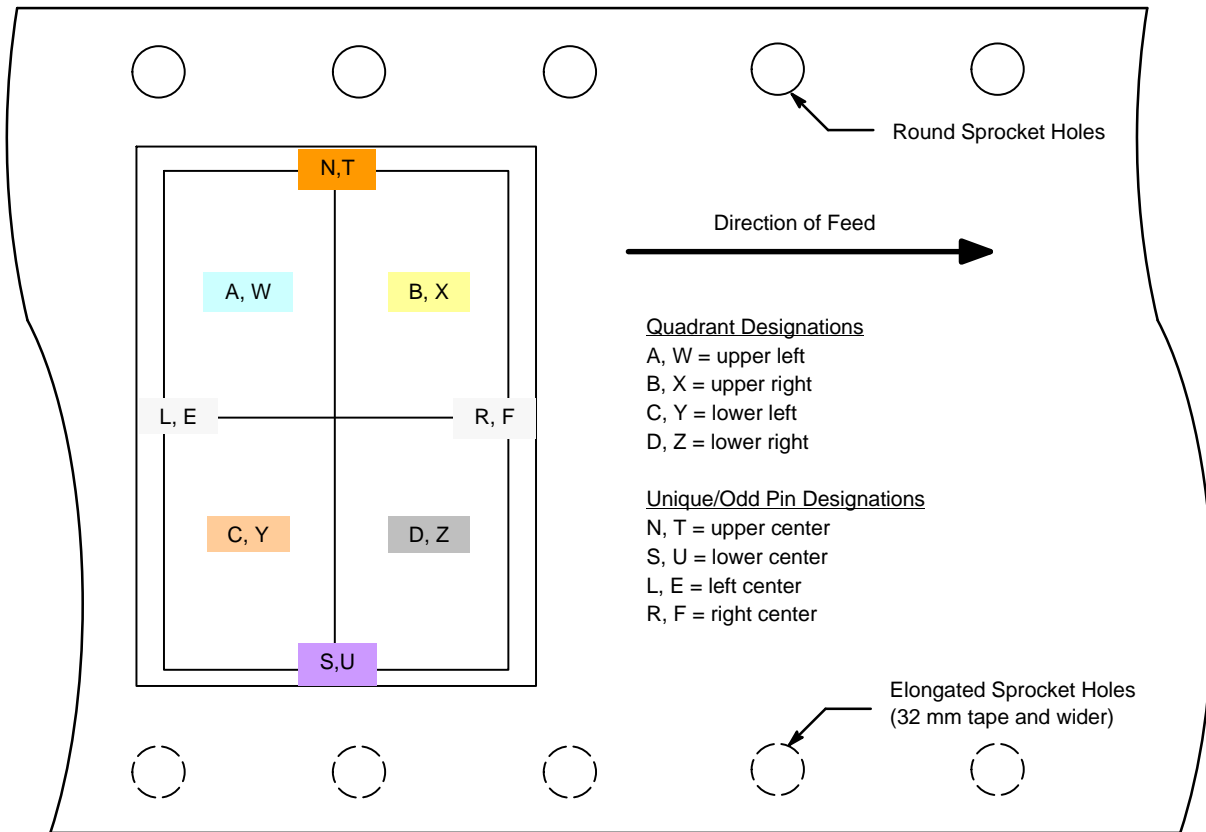
Figure 46. Leadless Package Pin 1 Orientation for Tape and Reel (Effective January 2007)
