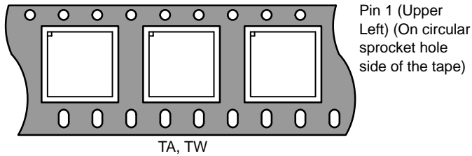
Figure 42. DFN/QFN (LPCC)/ WLCSP-4/XDFN2
