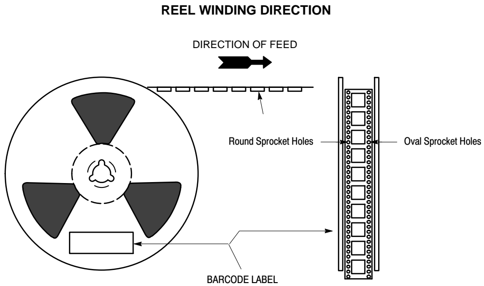
Figure 49. Round and Oval Sprocket Holes Used with 32 mm, 42 mm, 44 mm and 52 mm Tape (holes on both sides)
