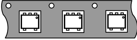
Figure 20. SOT-553 Option 1
