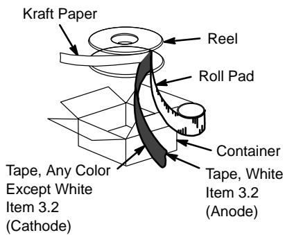
Figure 62. Reel Packing
