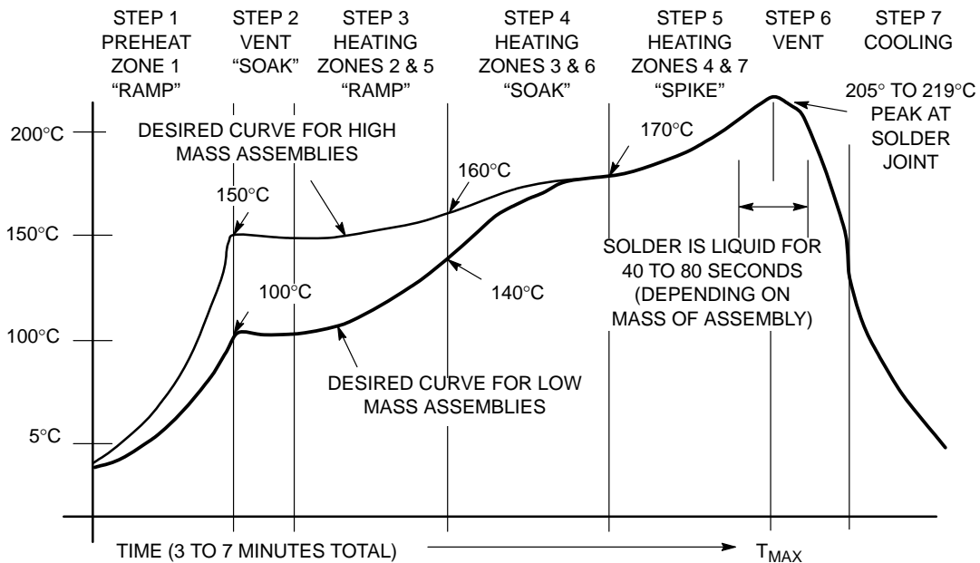
Figure 69. Typical Tin Lead (SnPb) Solder Heating Profile
