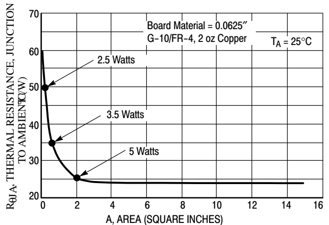
Figure 67. Thermal Resistance versus Drain Pad Area for the D²PAK Package (Typical)
