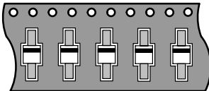
Figure 24. POWERMITE® "T1" Suffix – Option 1
