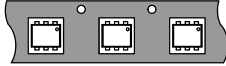
Figure 21. SOT-563 Option 1
