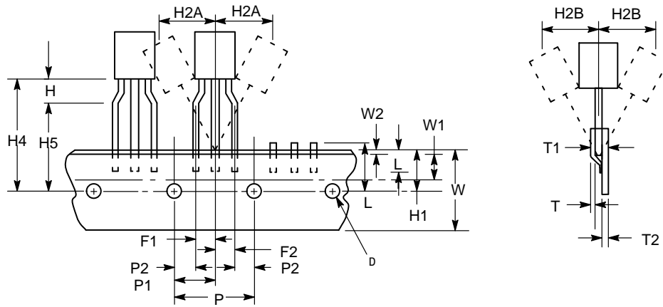
Figure 52. Device Positioning on Tape
