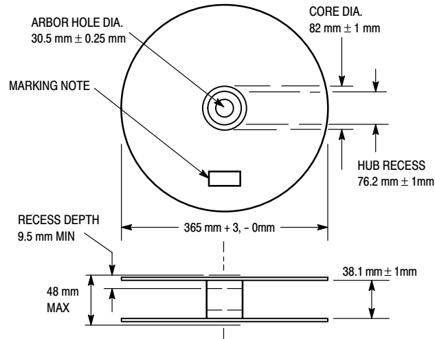
Figure 59. Reel Specifications
