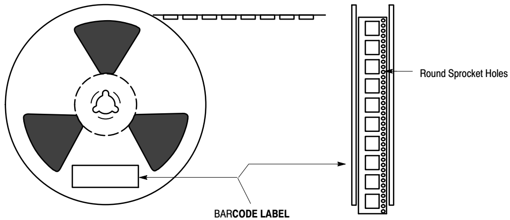
Figure 50. Round Sprocket Holes Used with 8 mm, 12 mm, 16 mm and 24 mm Tape (holes on one side only)
