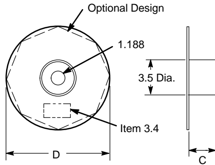
Figure 64. Reel Dimensions (Item references appear on Page 40)
