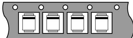
Figure 25. SMA, SMB, SMC "TR" or "R2" Suffix – Option 1, 3
