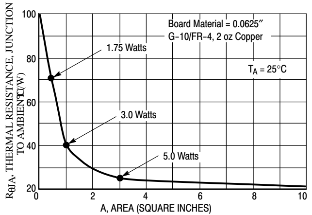
Figure 66. Thermal Resistance versus Drain Pad Area for the DPAK Package (Typical)
