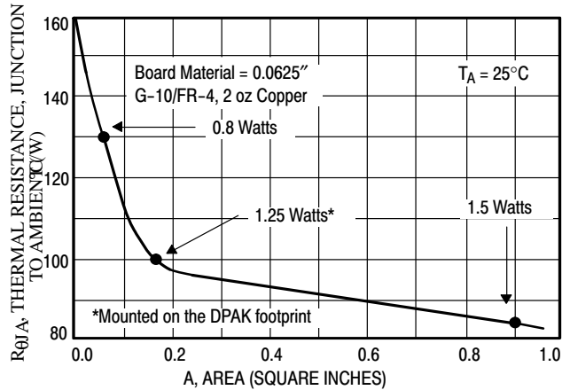
Figure 65. Thermal Resistance versus Drain Pad Area for the SOT-223 Package (Typical)
