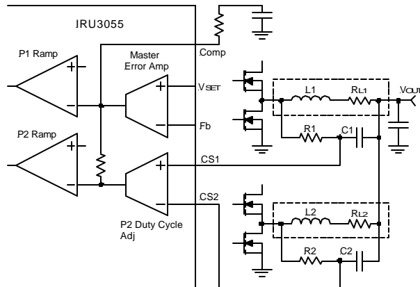
Figure 7 - Loss-less inductive current sensing and current sharing.
