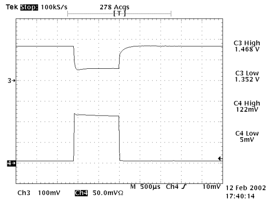
Figure 25 - 60A Load dynamic with 20A/μs slew rate. Ch4: Output current, sensed through 2mΩ resistor, 25A/div. Ch3: Ouput voltage, DC offset 1.3V, 100mV/div.
