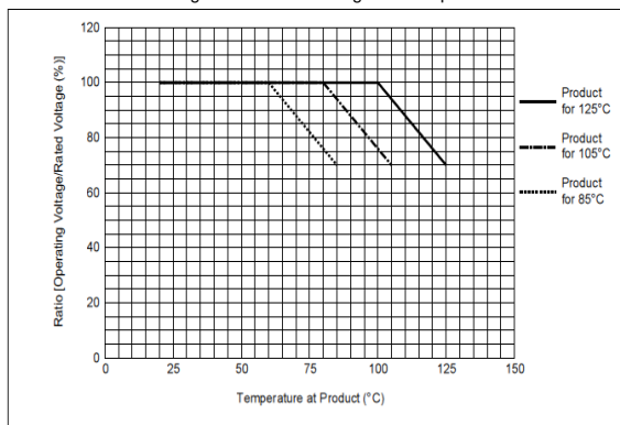
Recommended derating conditions on voltage and temperature
