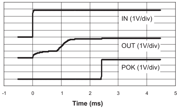
Power-Up With 1mA Load
