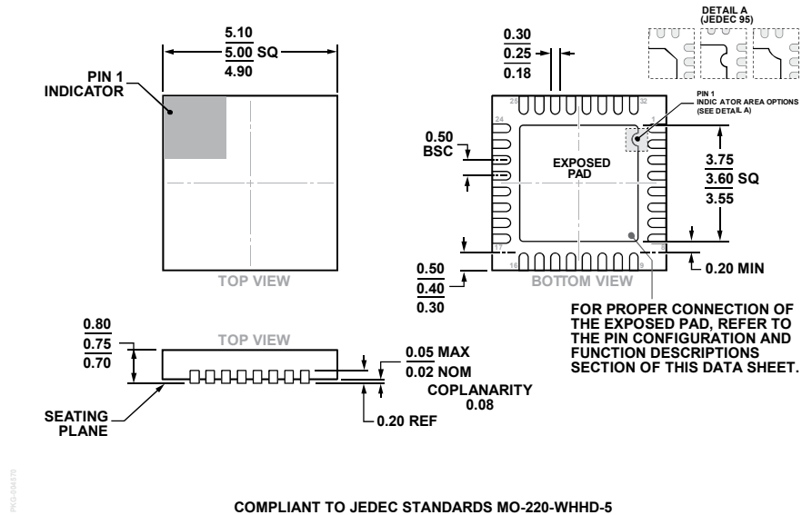
COMPLIANT TO JEDEC STANDARDS MO-220-WHHD-5 Figure 61. 32-Lead Lead Frame Chip Scale Package [LFCSPP] 5 mm x 5 mm Body and 0.75 mm Package Height (CP-32-12) Dimensions shown in millimeters
