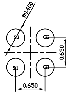
RECOMMENDED LAND PATTERN
