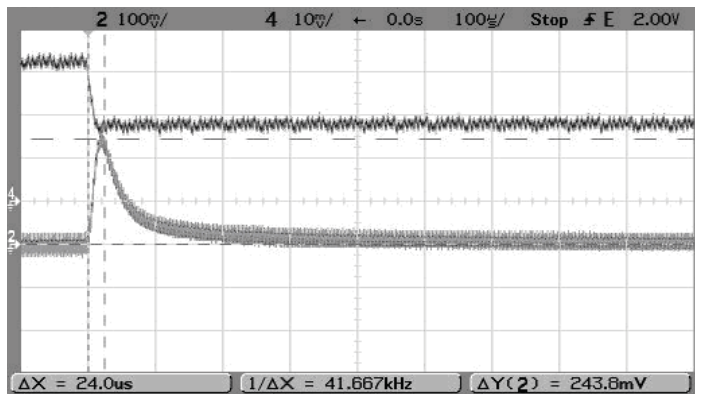
Step Load Transient Response (V IN =24V, V OUT =4.5V, C LOAD =0, I OUT =3A to 1.5A) Trace 2=V OUT , 100 mV/div. Trace 4=I OUT , 1A/div.
