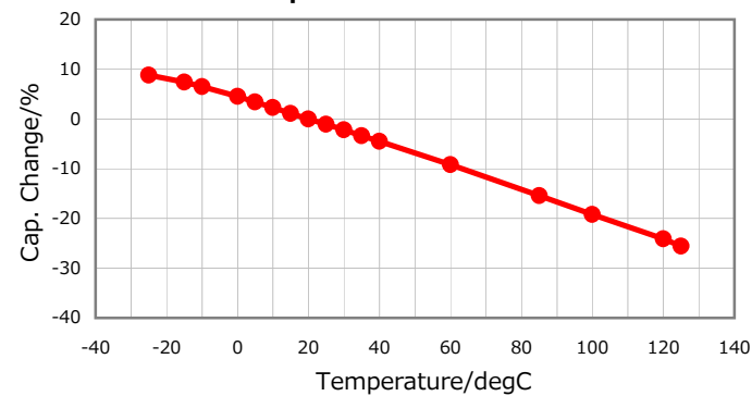
Temperature Characteristic
