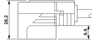
Valve connector, type A, side view
